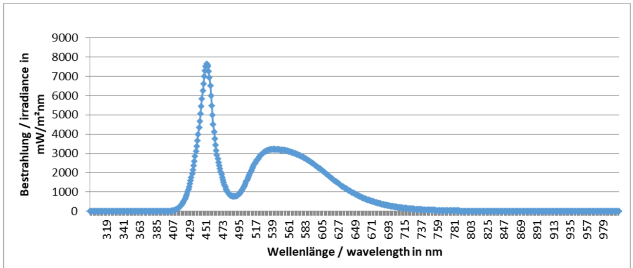
Fig. 1: Spectrum of LEDs
